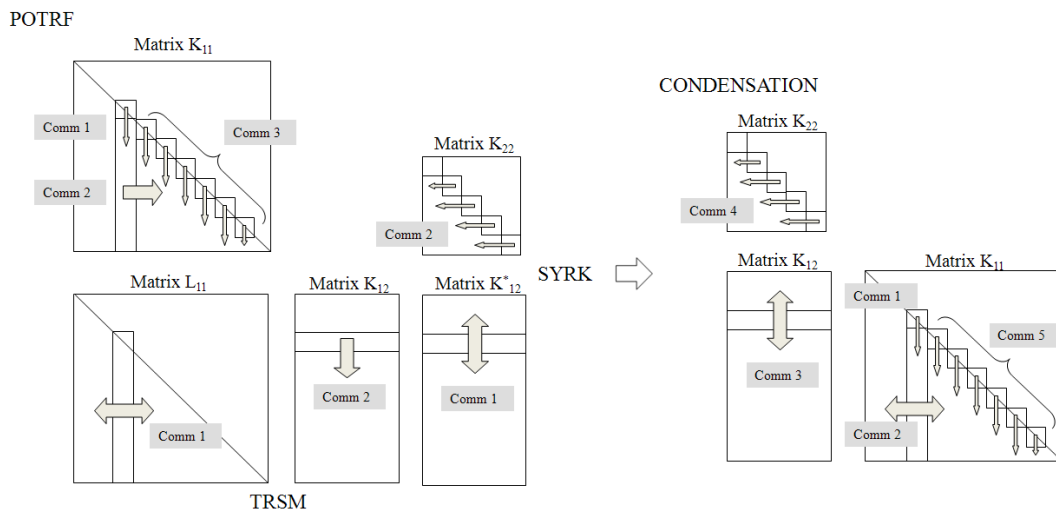
FIGURE 3. Communication pattern of each subroutine
