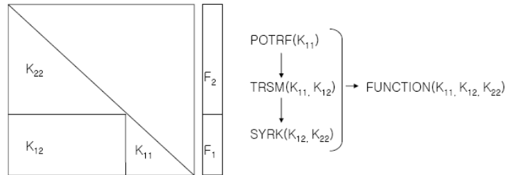
FIGURE 2. Frontal matrix and factorization routines
