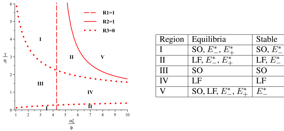
FIGURE 2. Regions and classification of Equilibria Stability with \alpha = 0.5 , \delta = 0.15 , \xi = 3 , \gamma = 0.1 , \phi = 0.25 , and \eta = 0.02
